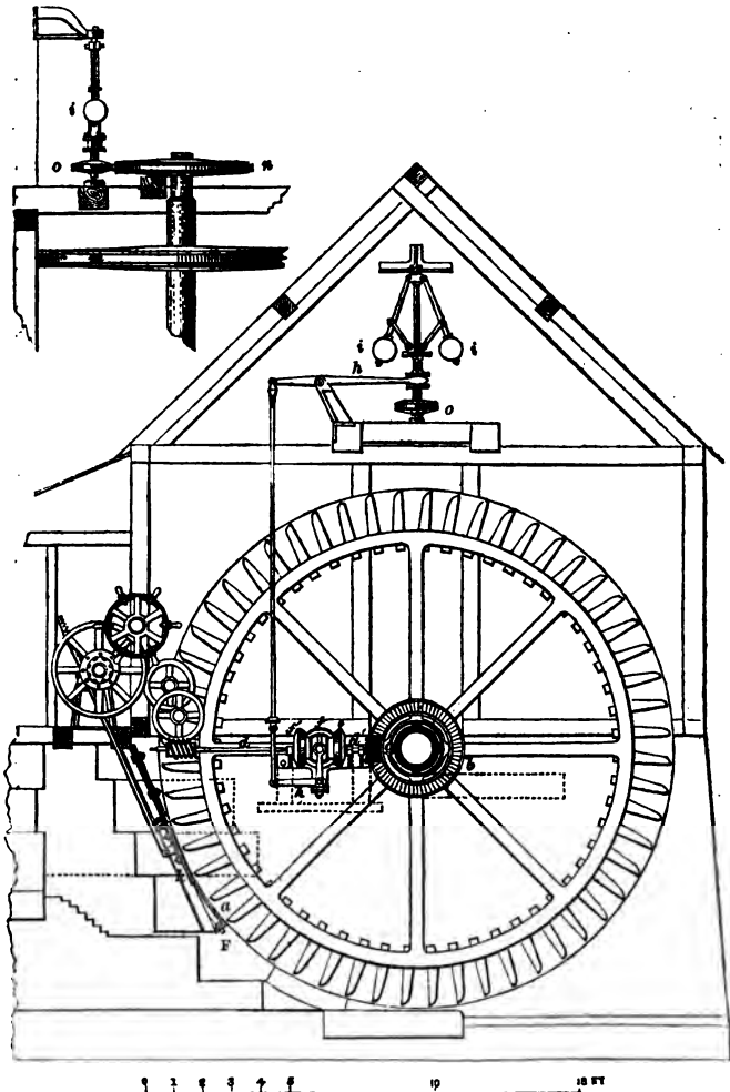
WATER-WHEEL AT WALTHAM ABBEY.
